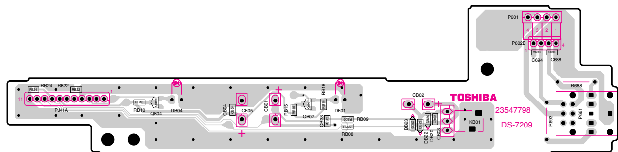
LED/RMT BOARD PD2119A2 (U005)
